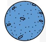
NEPTUNE
