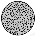
MERCURY
