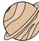
SATURN
